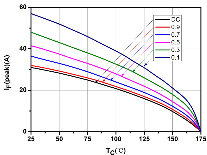
Fig.8-Current Derating
