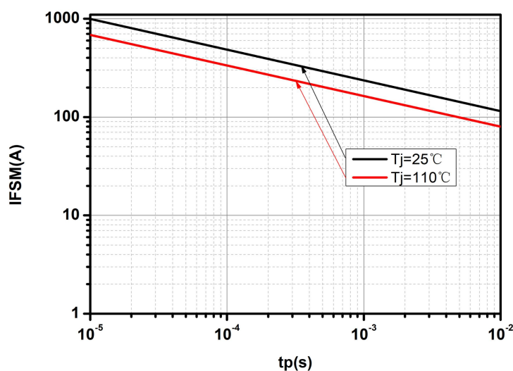
Fig.6-Non-repetitive peak forward surge current versus pulse duration (sinusoidal waveform)
